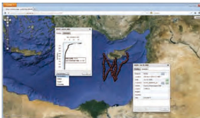
Fig. 1 - Example of vertical profile and metadata from a glider station in the Levantine Basin.
