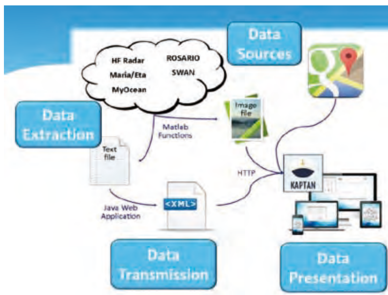
Fig. 2 - Schematic of data flow: sourcing and extraction from observing and modelling platforms to data transmission and presentation on the web and smartphone interfaces.
