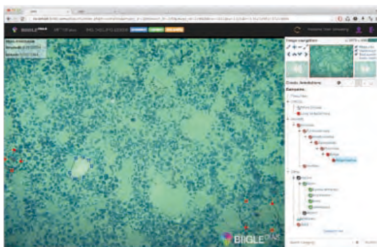
Fig. 3 - Annotation System.
